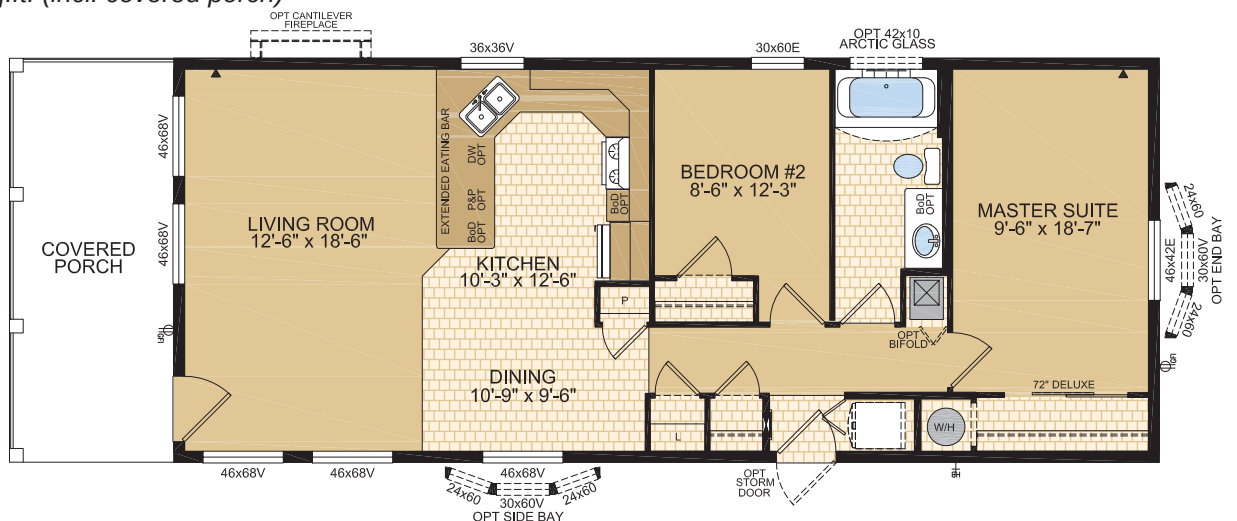
OPTIONAL KITCHEN
